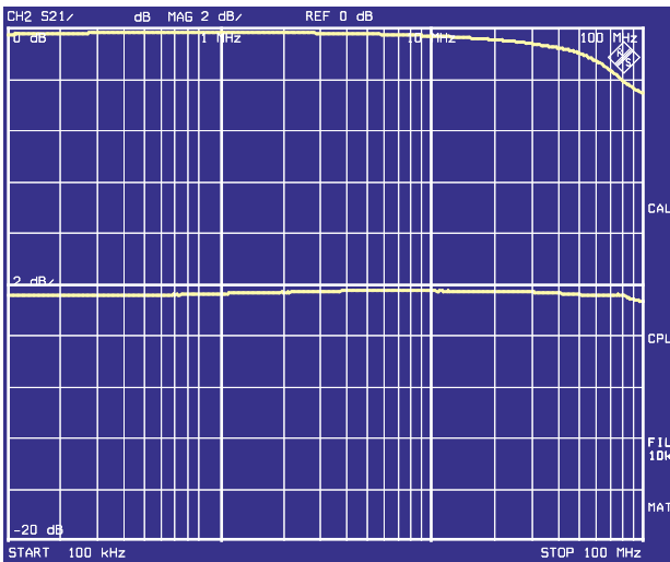
Fig. 1: The insertion loss of the symmetrical circuit, measured with a line impedance of 100 \Omega (upper curve), determines the transmission bandwidth of the network for the useful signal. The voltage-division factor (lower curve) is to be added to the measured voltage for the frequency range 150 kHz to 30 MHz for comparison with the emission limit
